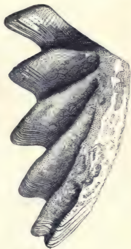
Fig. 89. Cer. runcinatus .
